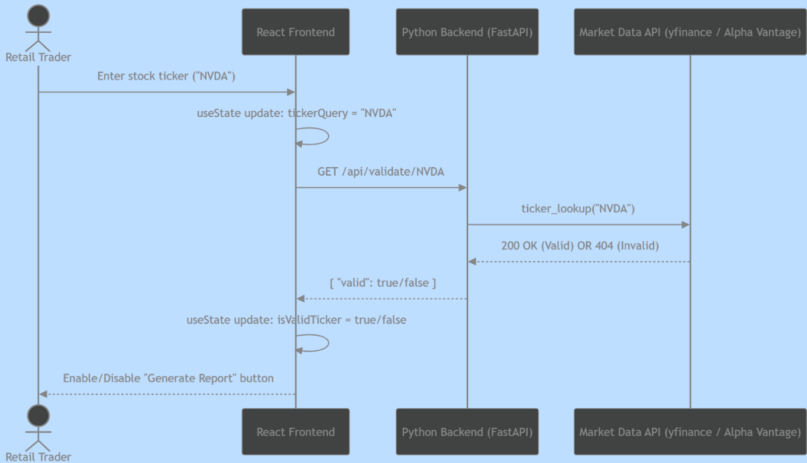
Sequence Diagram for Stock Ticker Lookup
